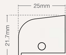
Window head trim end closer CL 023
