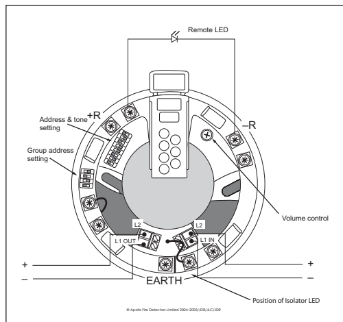
Fig. 2 Sounder Beacon Base with isolator wiring
