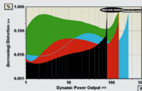
ABOVE: Dynamic power output versus distortion into 8ohm (black trace), 4ohm (red), 2ohm (blue) and 1ohm (green) speaker loads. Max. current is 12.1A
