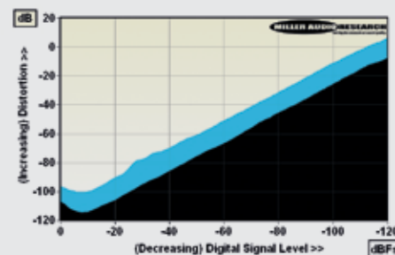
ABOVE: Distortion vs. 24-bit digital signal level over a 120dB range, fixed line out (1kHz, black; 20kHz, blue)
