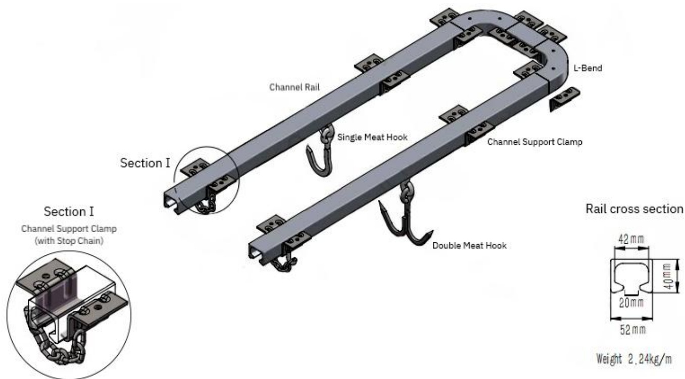
Figure 1: Sliding Rail System Schematic
